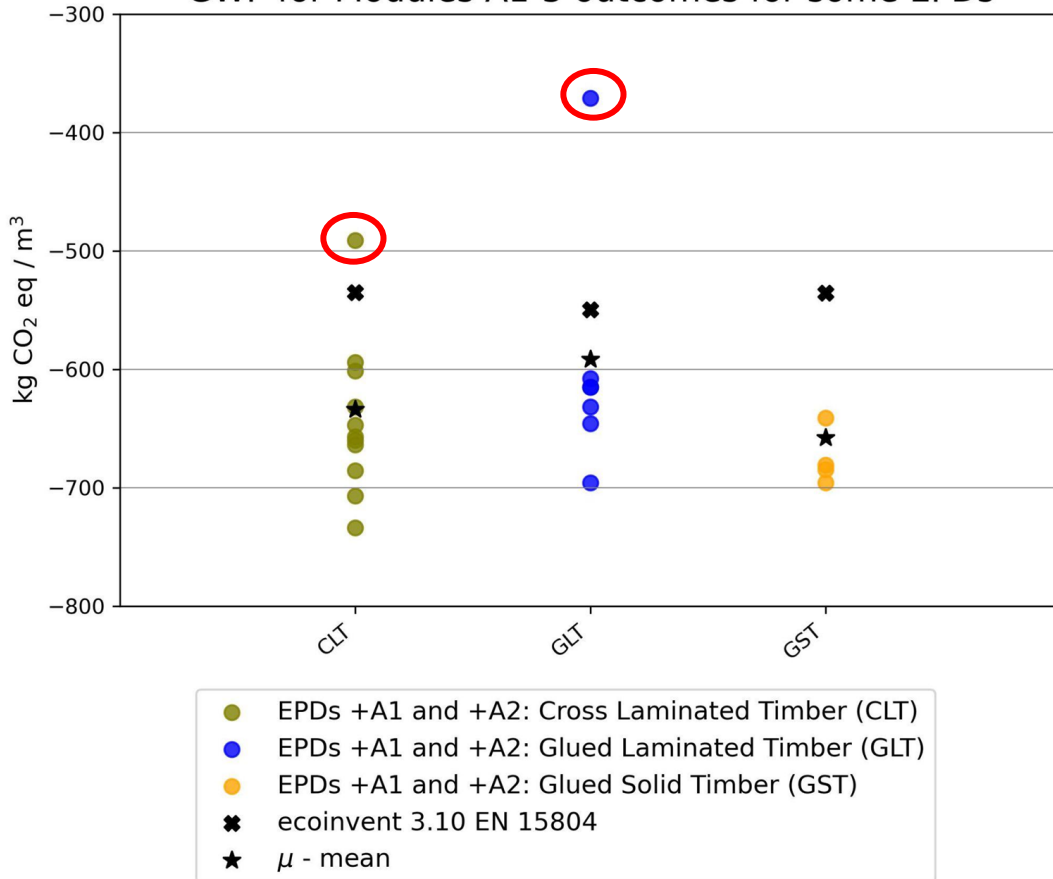
GWP for Modules A1-3 outcomes for some EPDs
